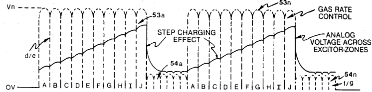
SECTION AA: APPLIED VOLTAGE PULSE TRAIN
